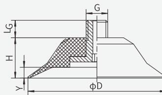
SPF5-50 Male thread connection
